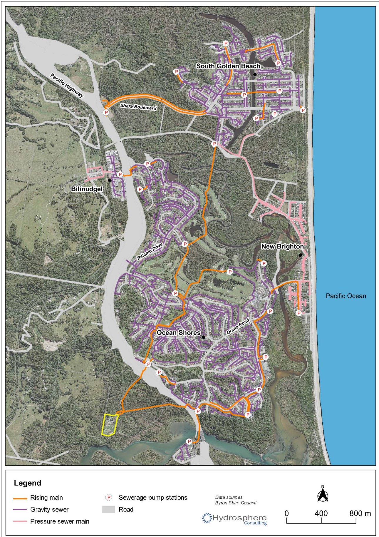
Figure 2: Ocean Shores sewerage network
