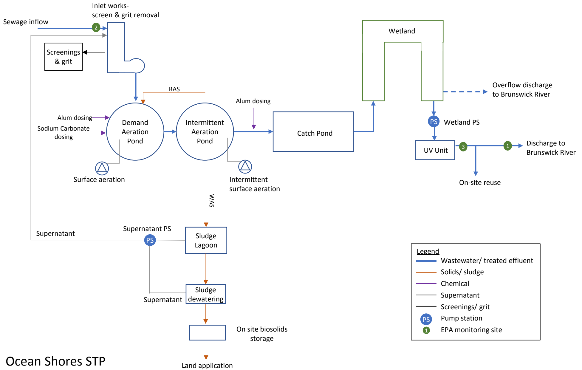
Figure 5: Ocean Shores STP process diagram
